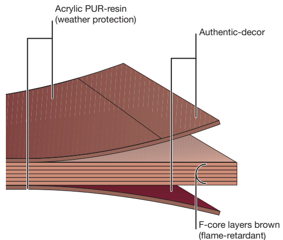
Structure Max Compact Laminate „Authentic“
